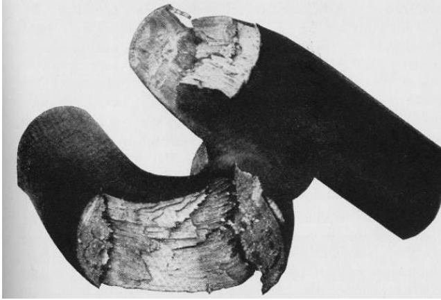
Wrought Iron nick bend test
