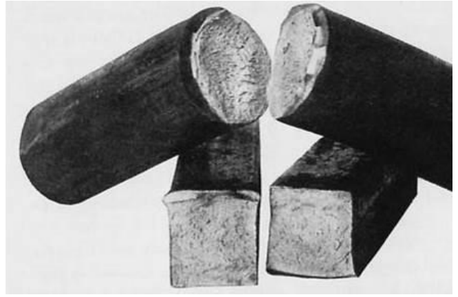
Mild Steel nick bend test
